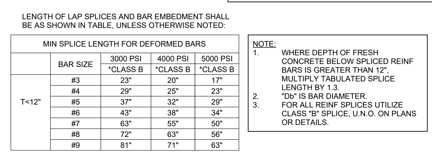
1 TYPICAL LAP SPLICE SCHEDULE 3/4" = 1'-0"
